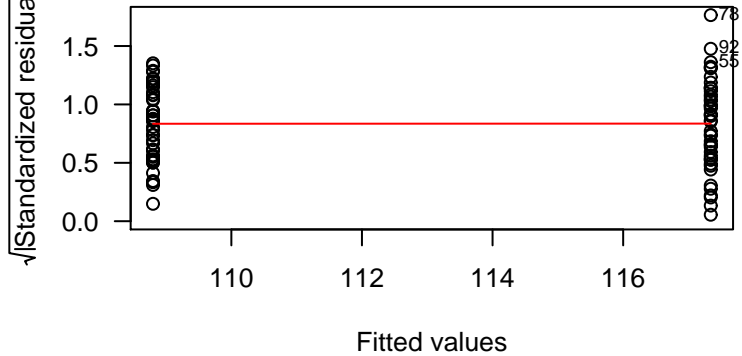
Scale-Location
