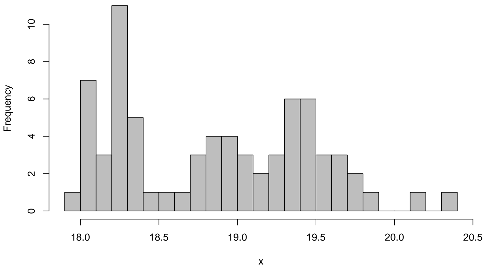
Histogram
