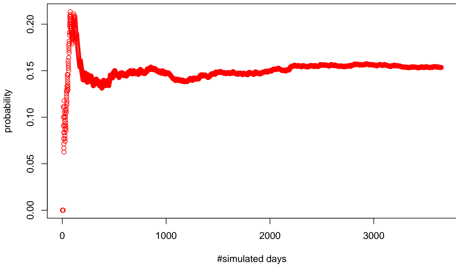
Probability in Small Hospital
