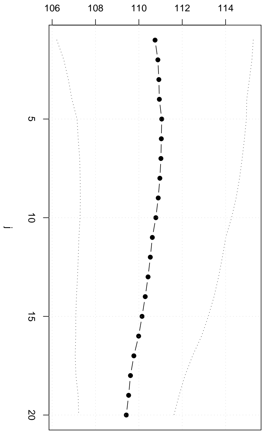
Trimmed Mean(j/n)
