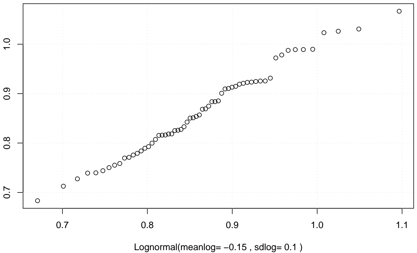
QQ plot (Lognormal)
