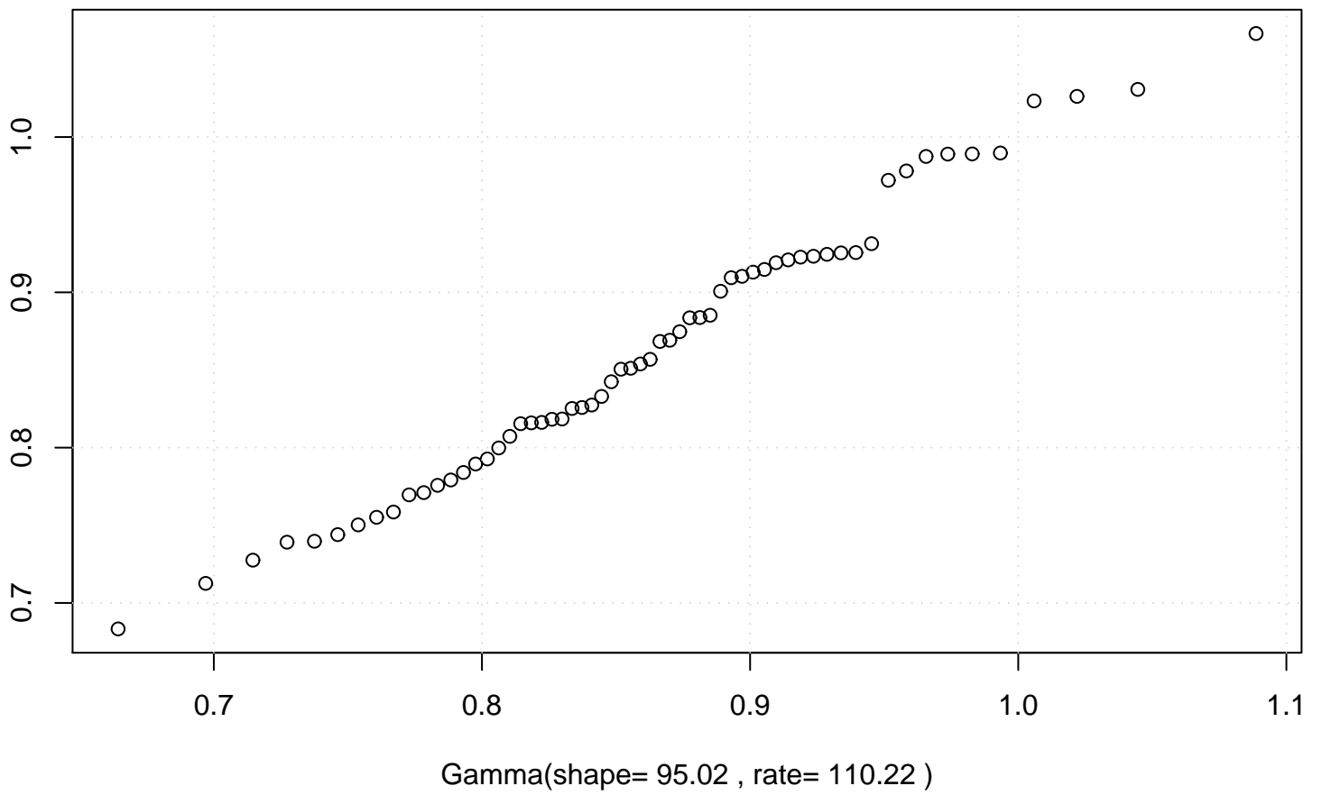
QQ plot (Gamma)
