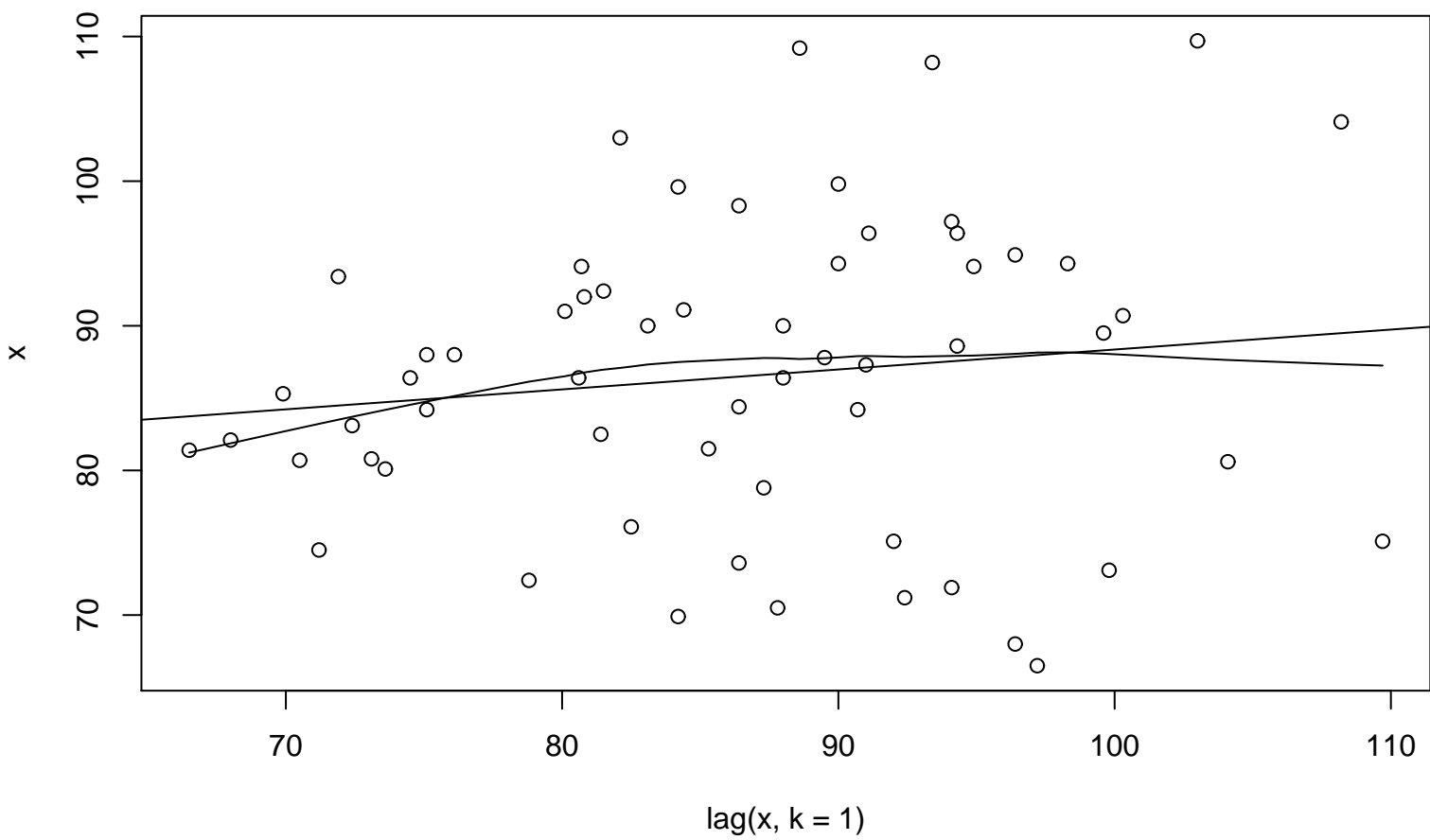
Lag plot, lowess, and regression line
