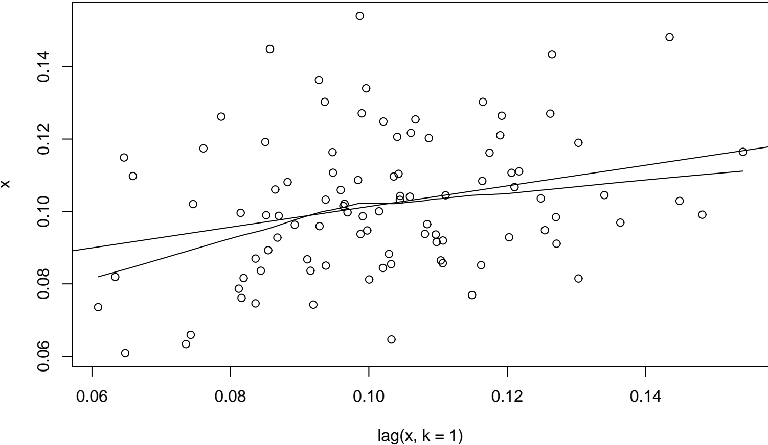
Lag plot, lowess, and regression line
