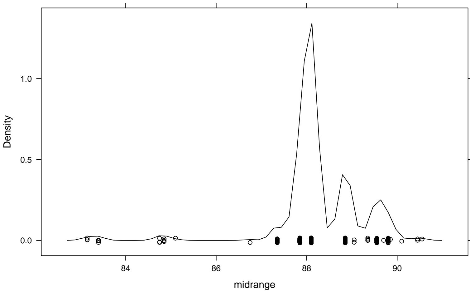
Density Plot
