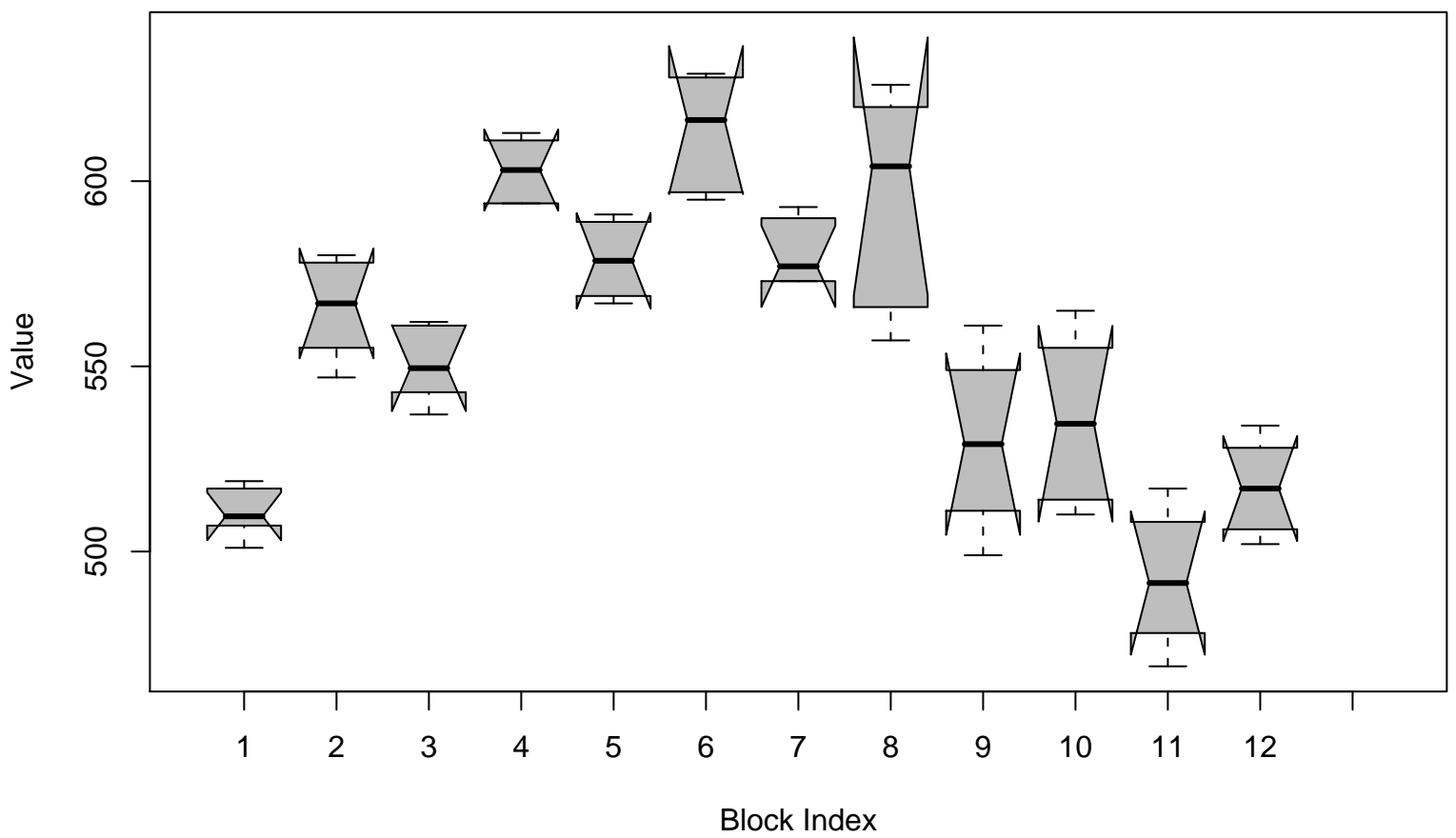
Notched Box Plots – Sequential Blocks
