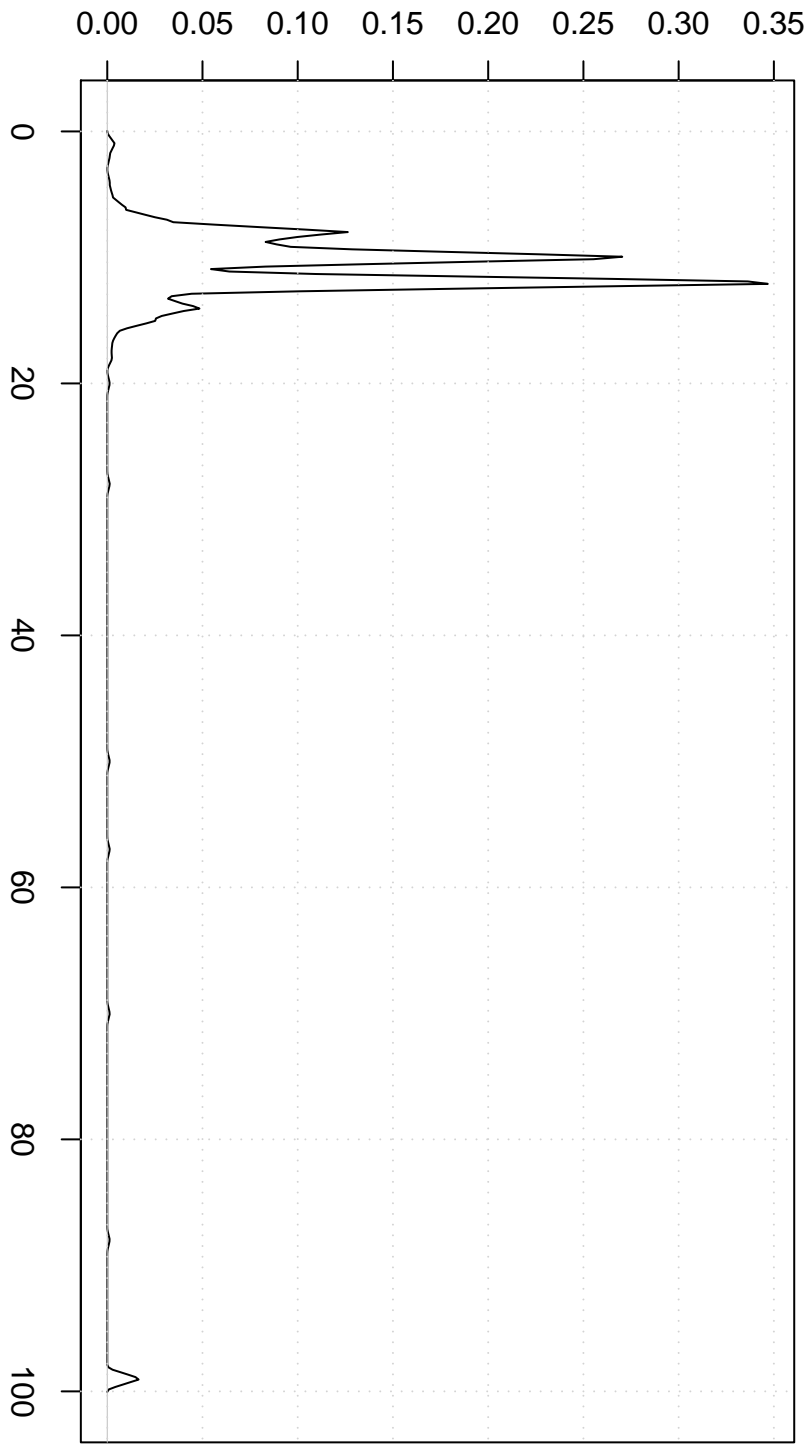
Triangular Kernel
