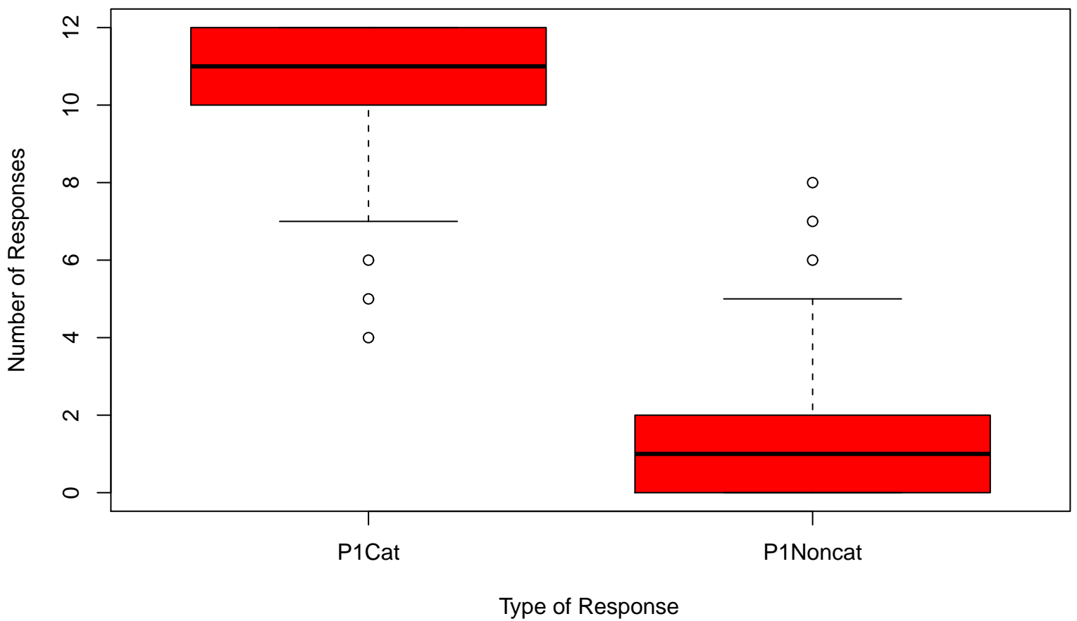
Fig 1 – Odd-One-Out Task
