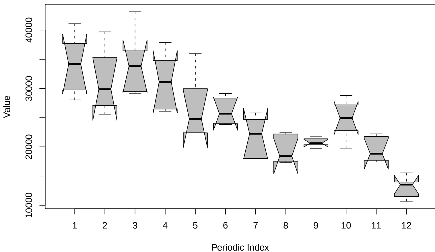
Notched Box Plots – Periodic Subseries
