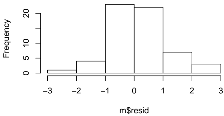
Residual Histogram
