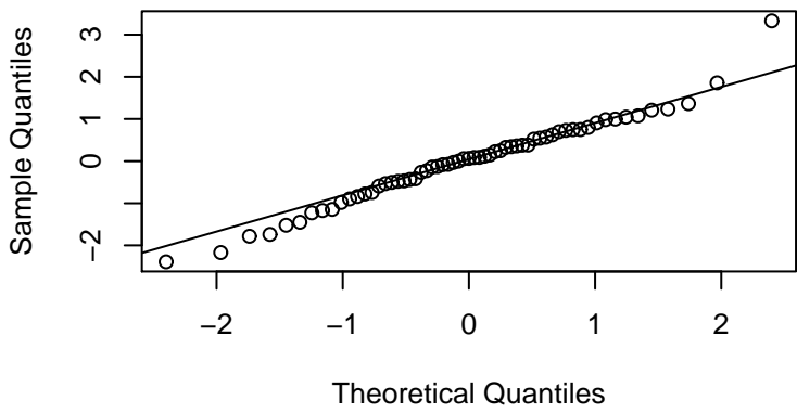
Residual Normal QQ Plot
