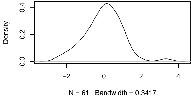
Residual Kernel Density
