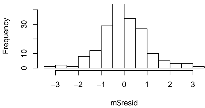
Residual Histogram
