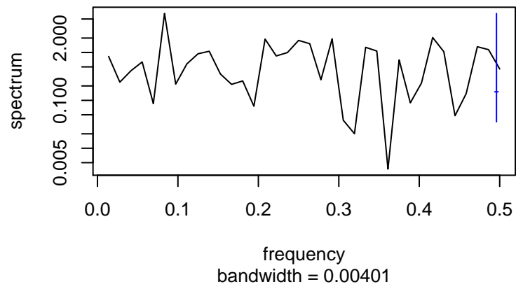
Standardized Residuals
