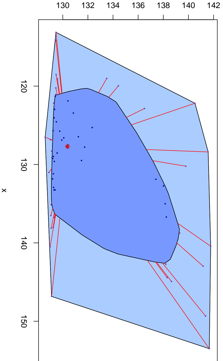
Bagplot
