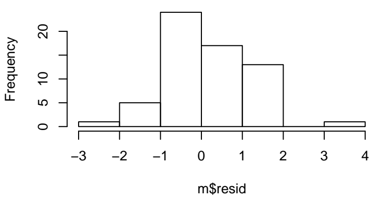
Residual Histogram
