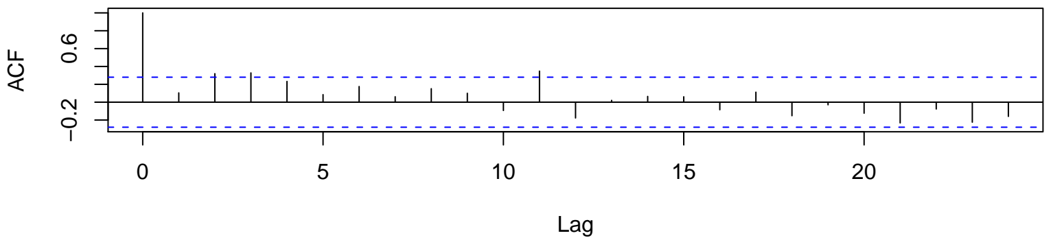
ACF of x (transformed and differenced)
