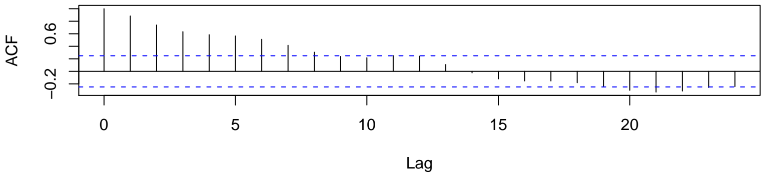
ACF of x (raw)
