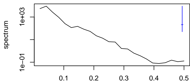
frequency bandwidth = 0.00601
