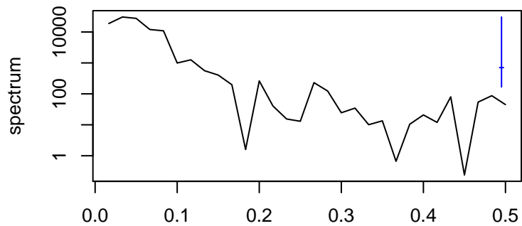
frequency bandwidth = 0.00481
