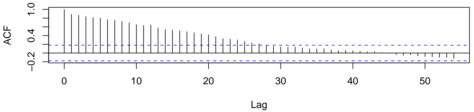
ACF of x (raw)
