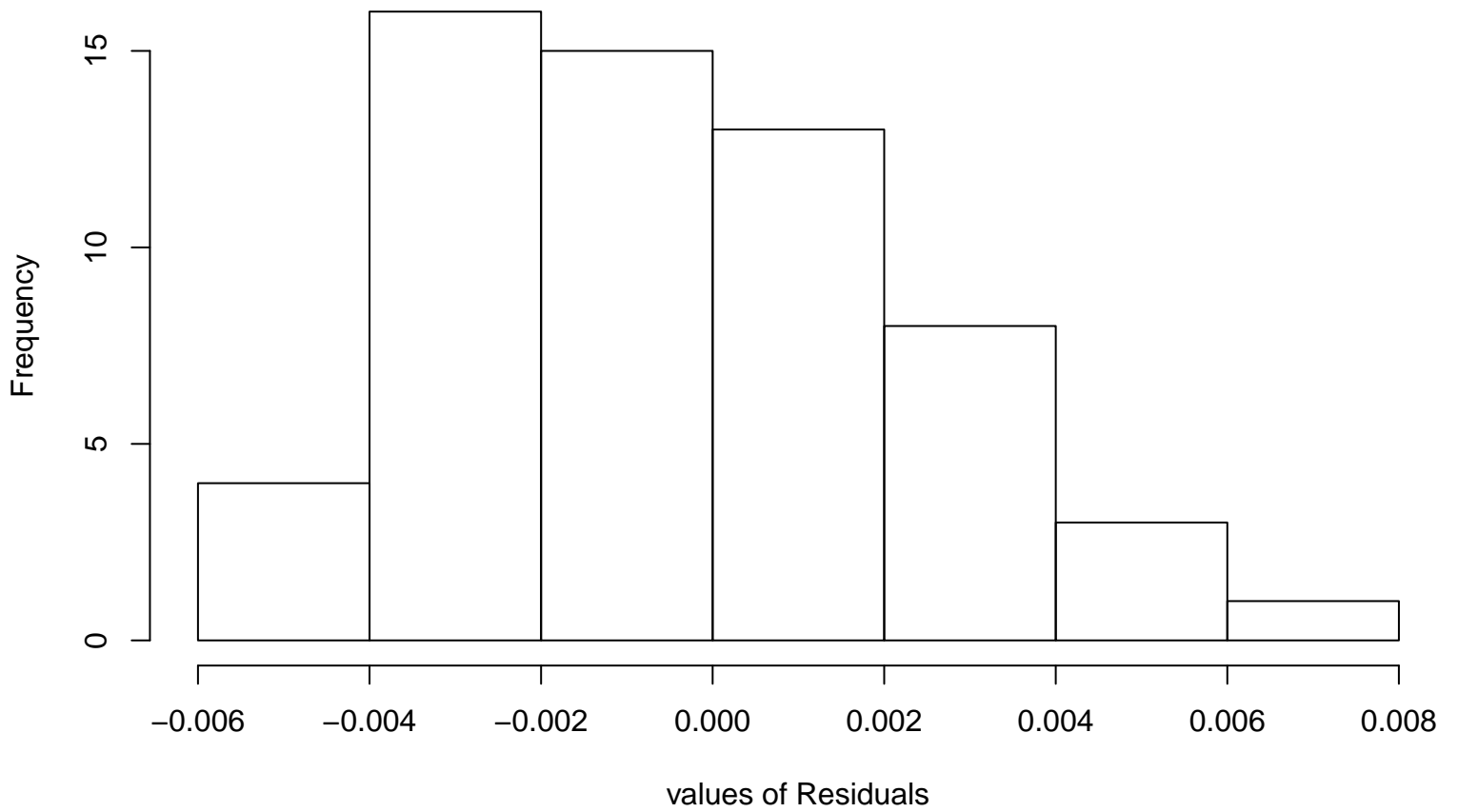
Residual Histogram
