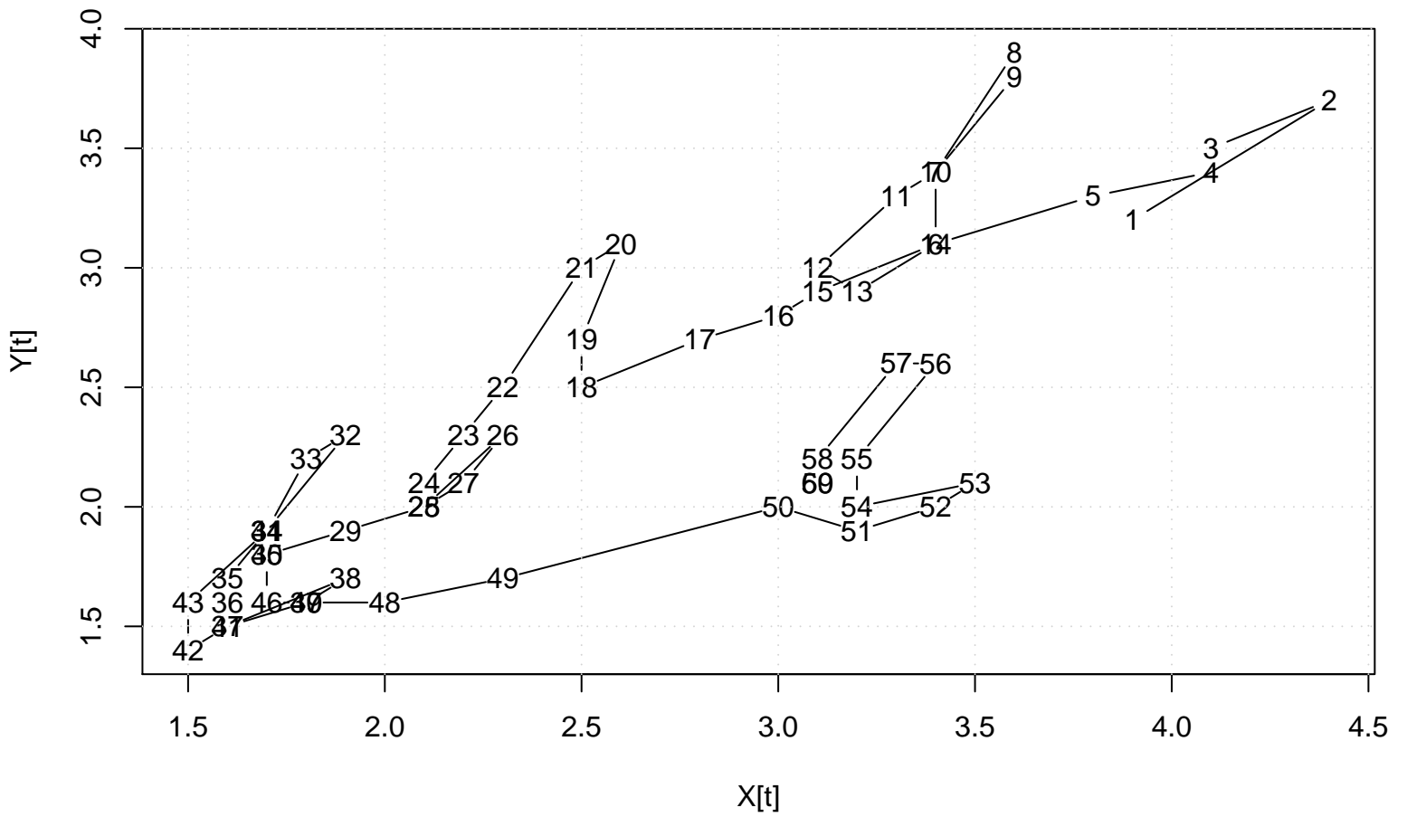
Scatter Plot
