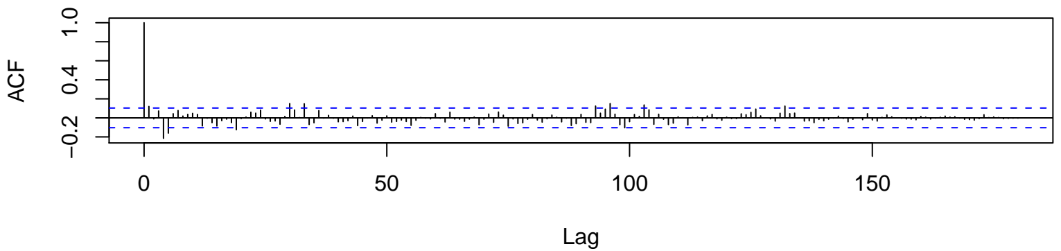
ACF of x (transformed and differenced)
