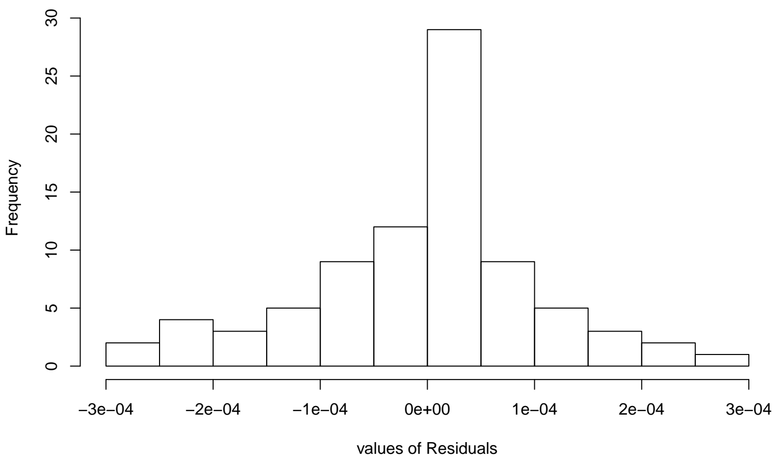
Residual Histogram
