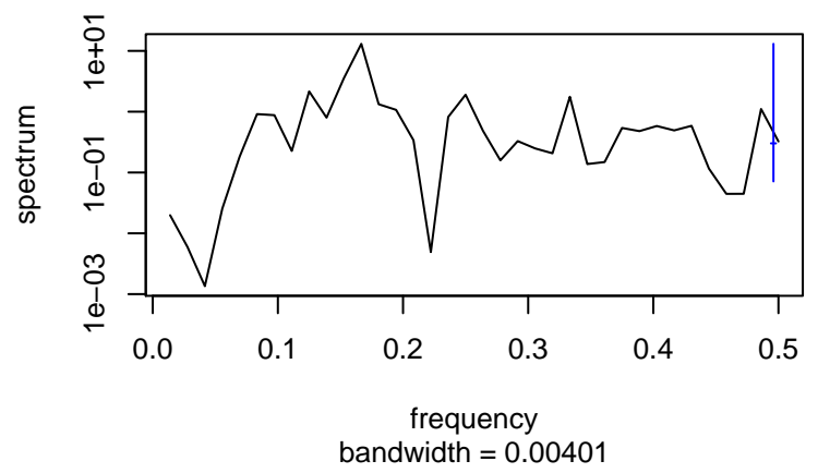
Standardized Residuals
