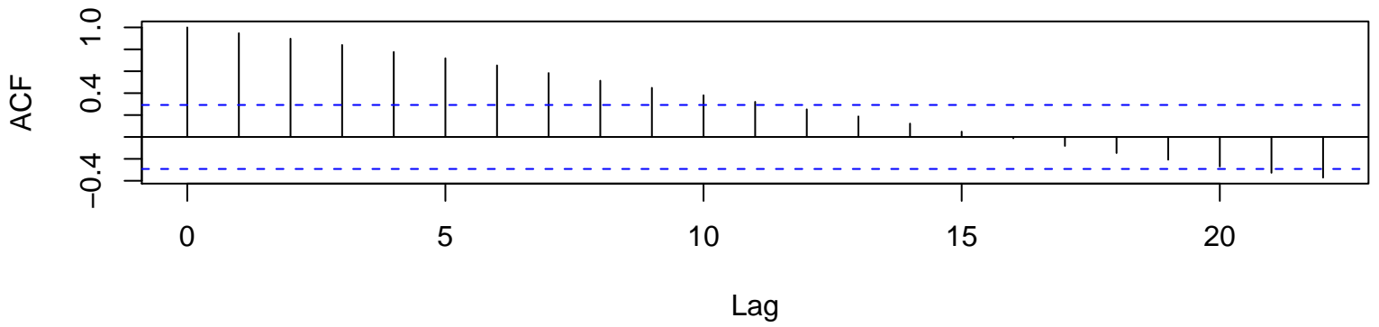
ACF of y (raw)
