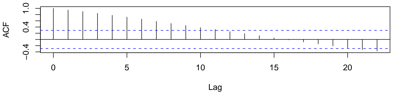
ACF of y (transformed and differenced)
