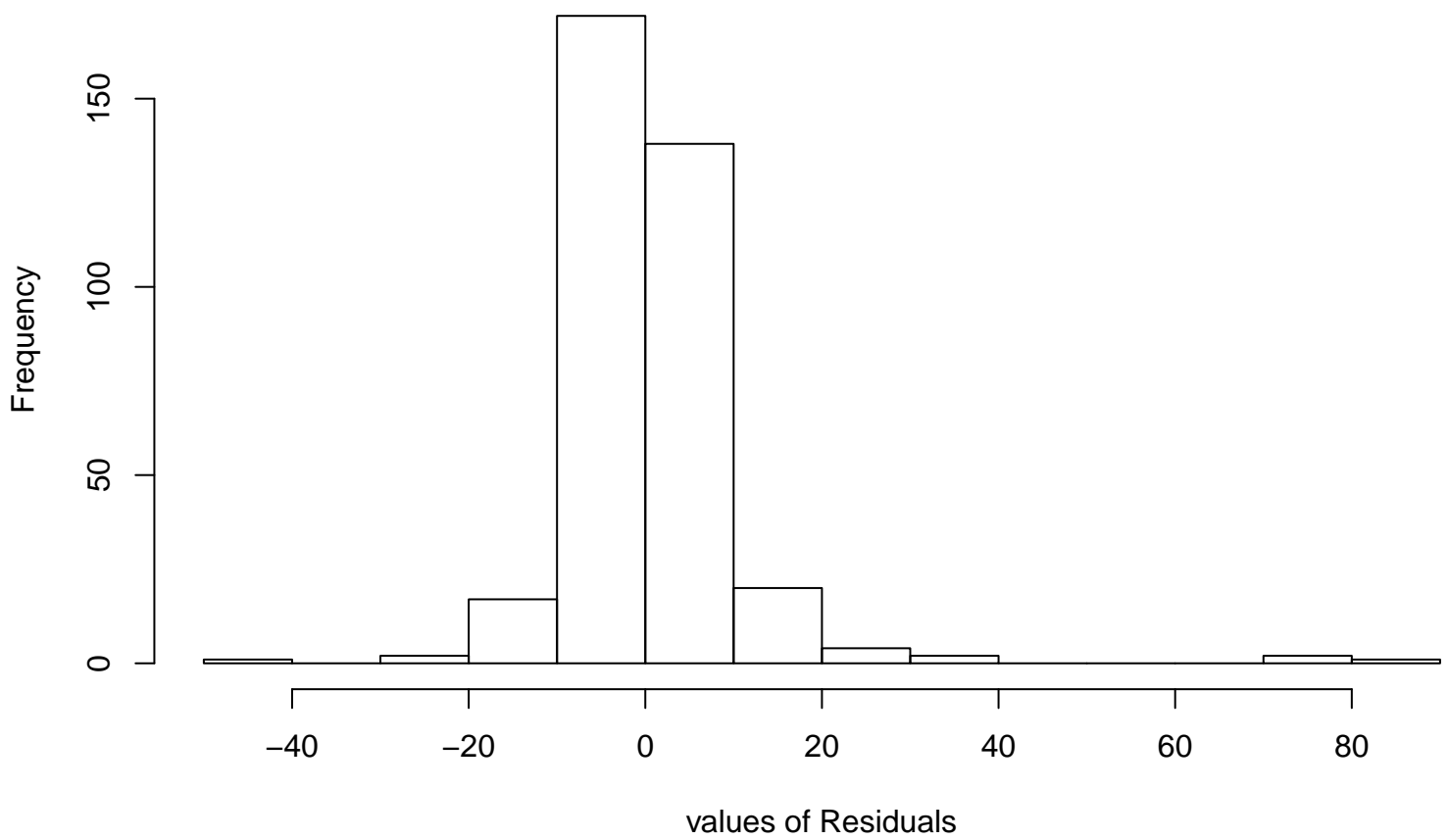
Residual Histogram
