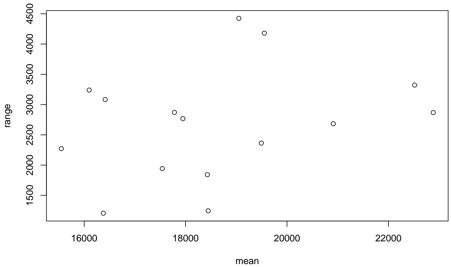
Range-Mean Plot
