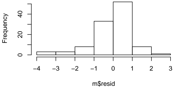
Residual Histogram
