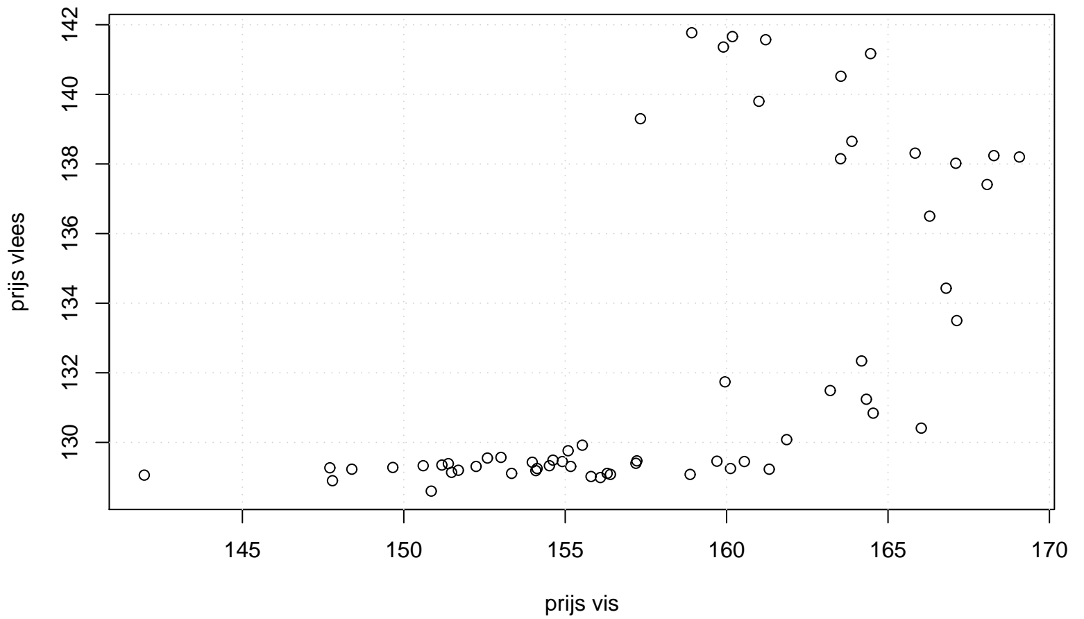
Scatterplot
