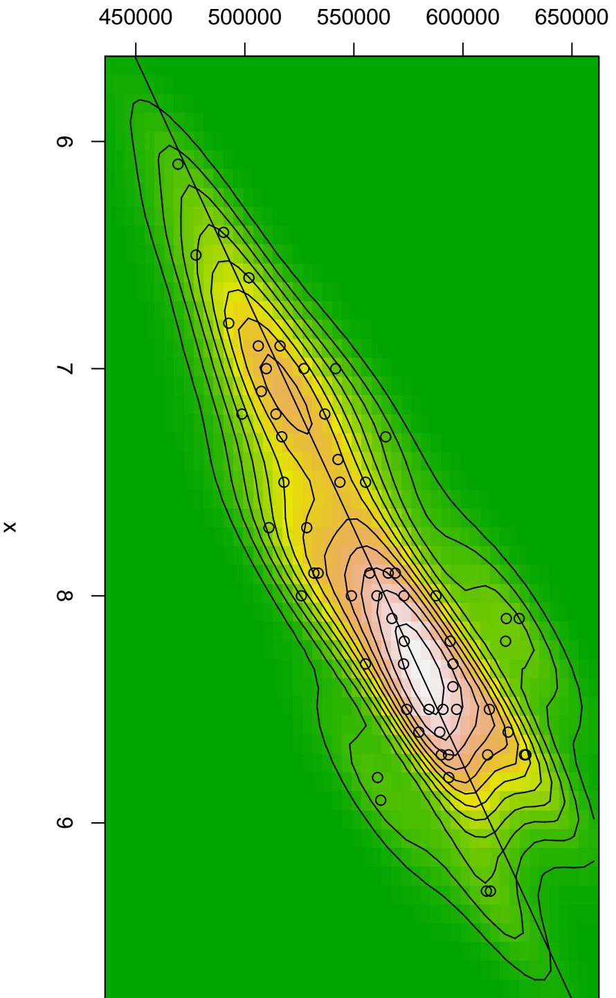
Bivariate Kernel Density
