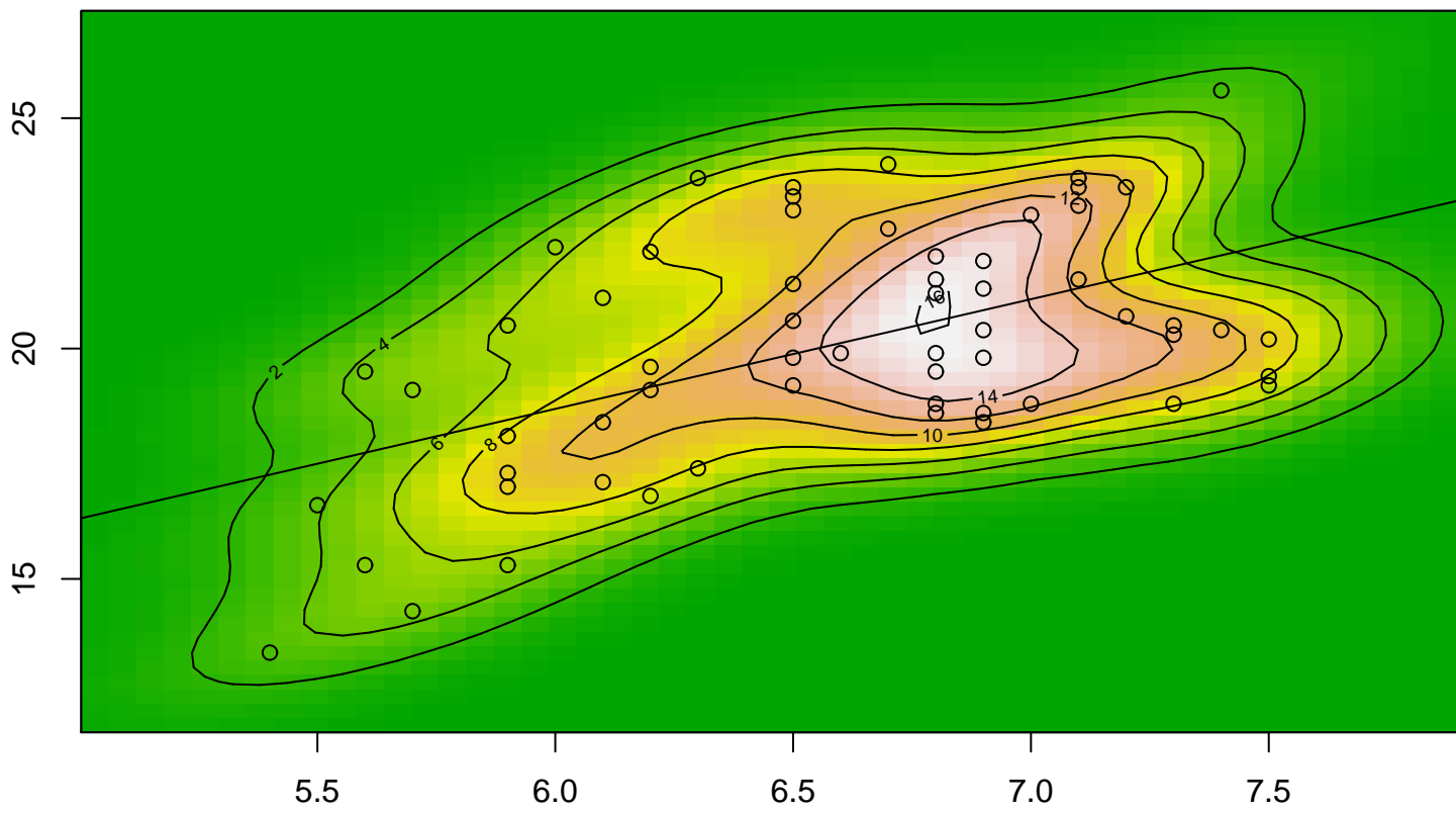
Bivariate Kernel Density Plot (x,y)
