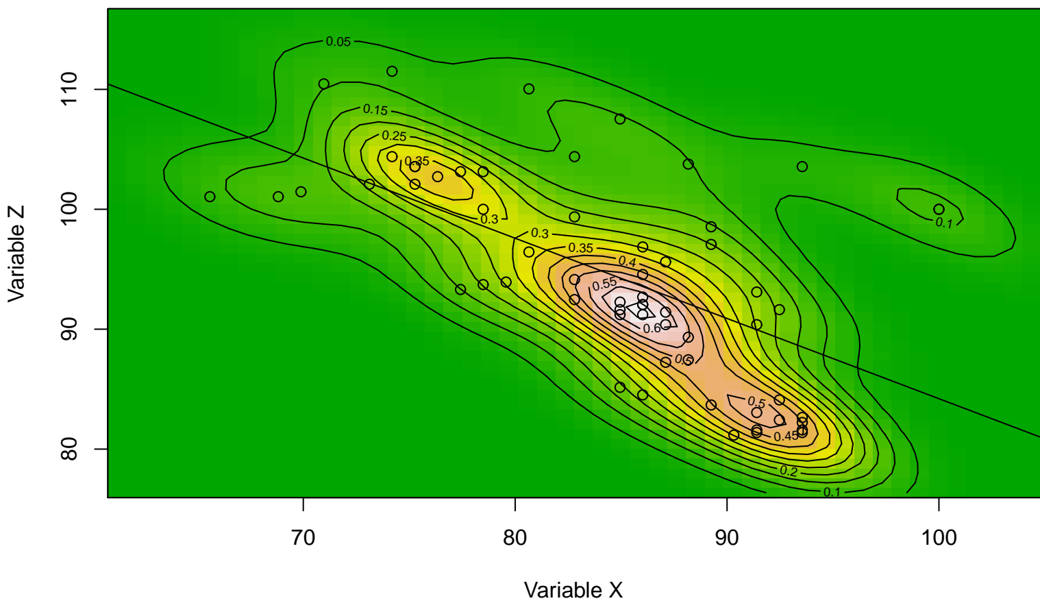
Bivariate Kernel Density Plot (x,z)
