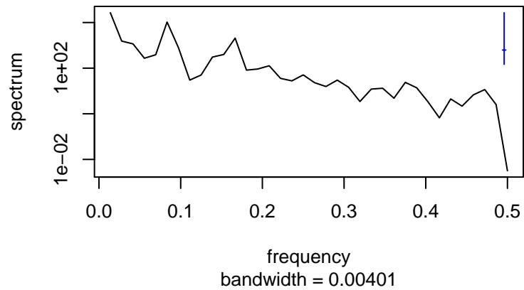
Standardized Residuals
