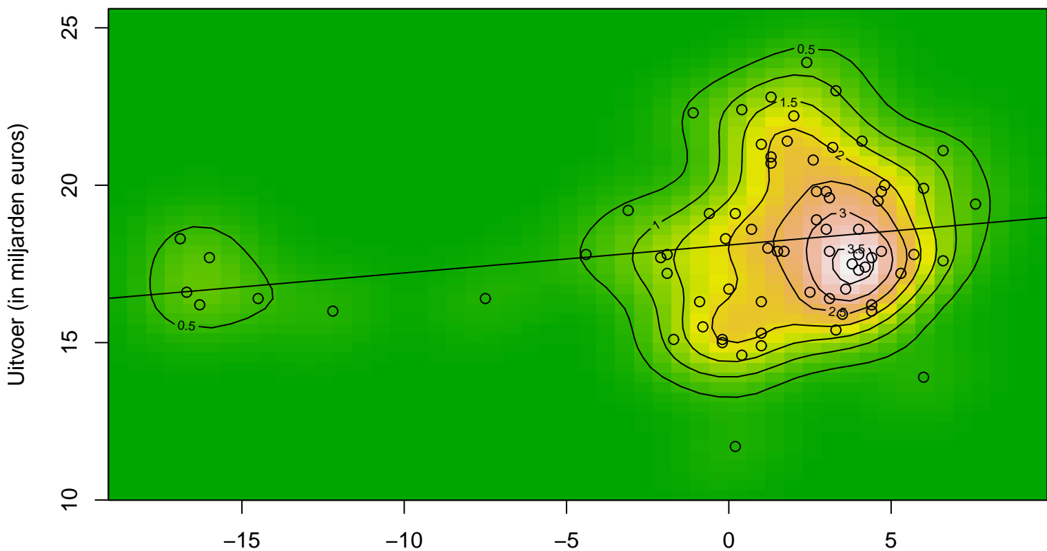
Bivariate Kernel Density Plot (x,y)
