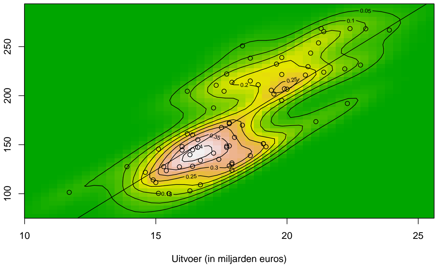
Bivariate Kernel Density Plot (y,z)
