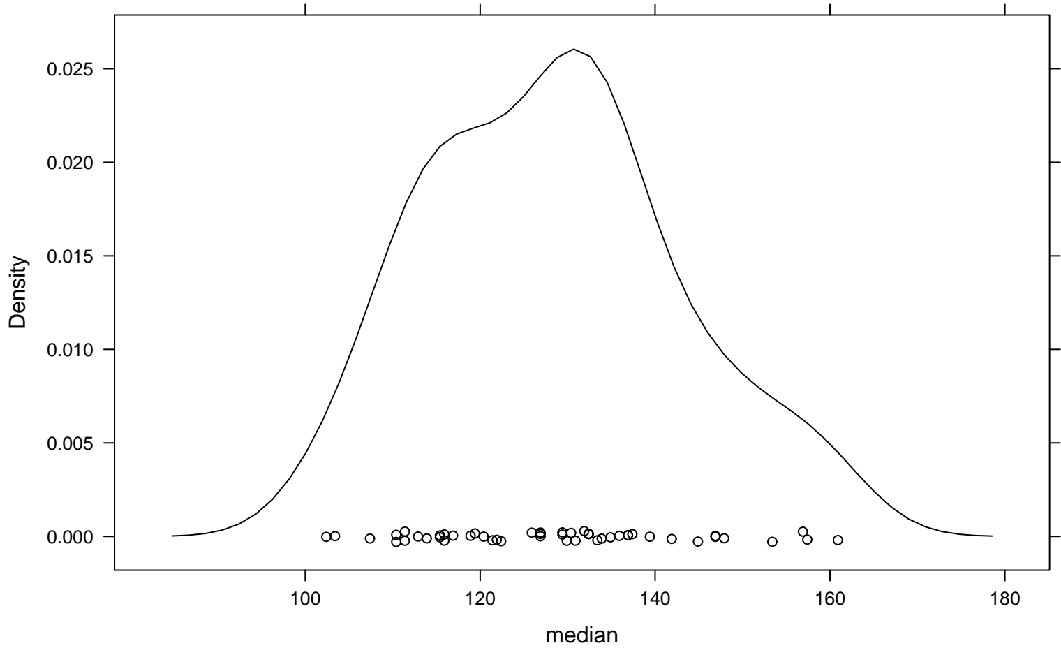
Density Plot
