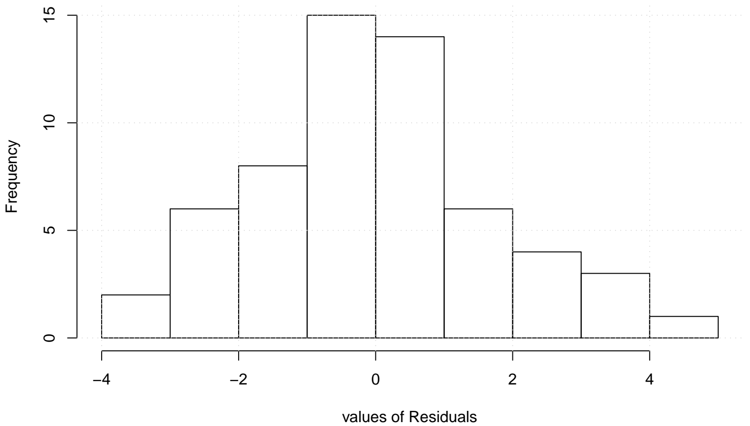
Residual Histogram
