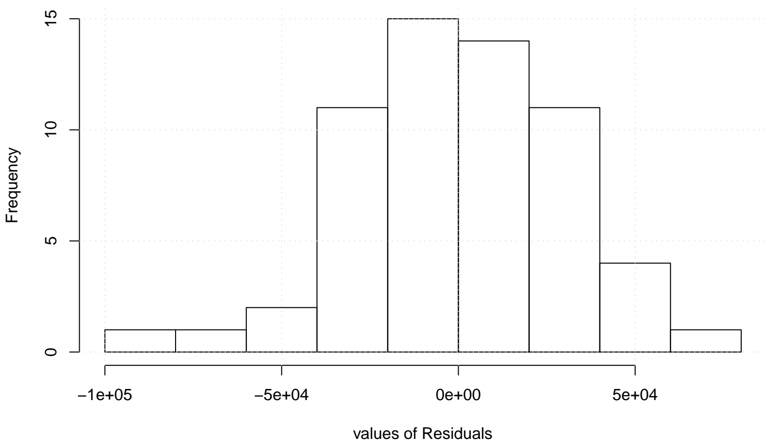
Residual Histogram
