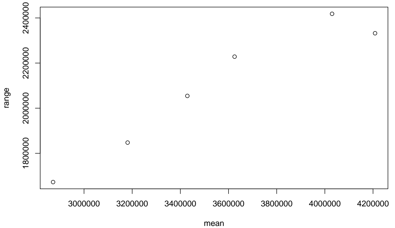
Range-Mean Plot
