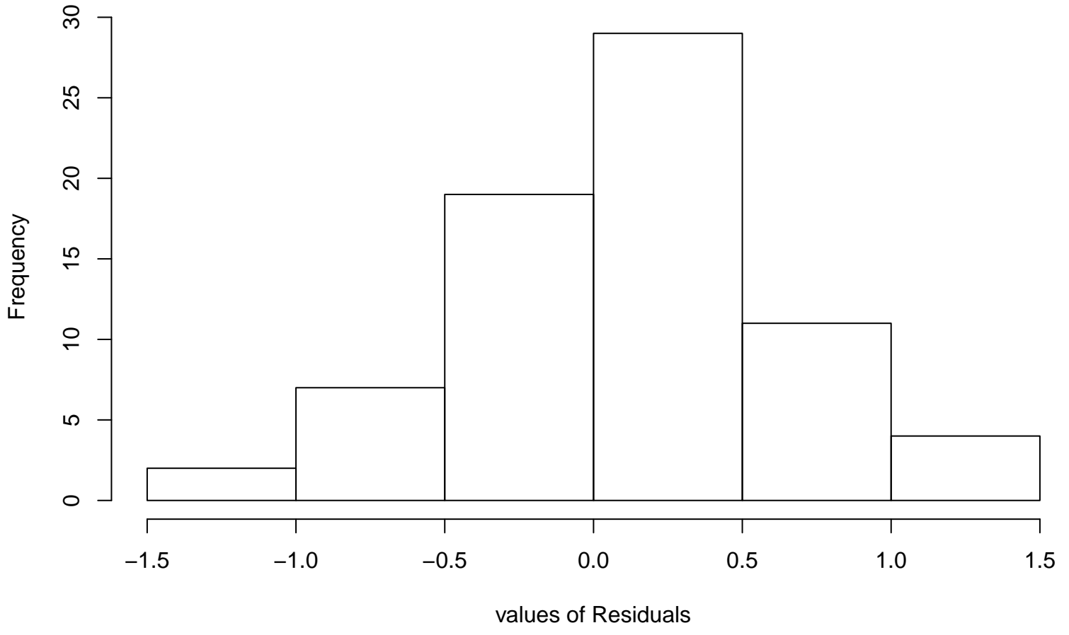
Residual Histogram
