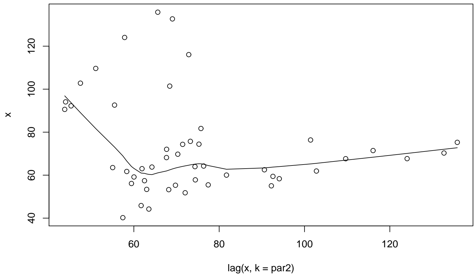
Lag plot (k=12), and lowess
