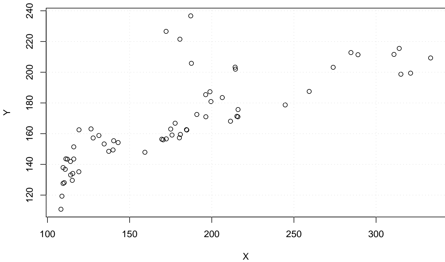
Scatterplot
