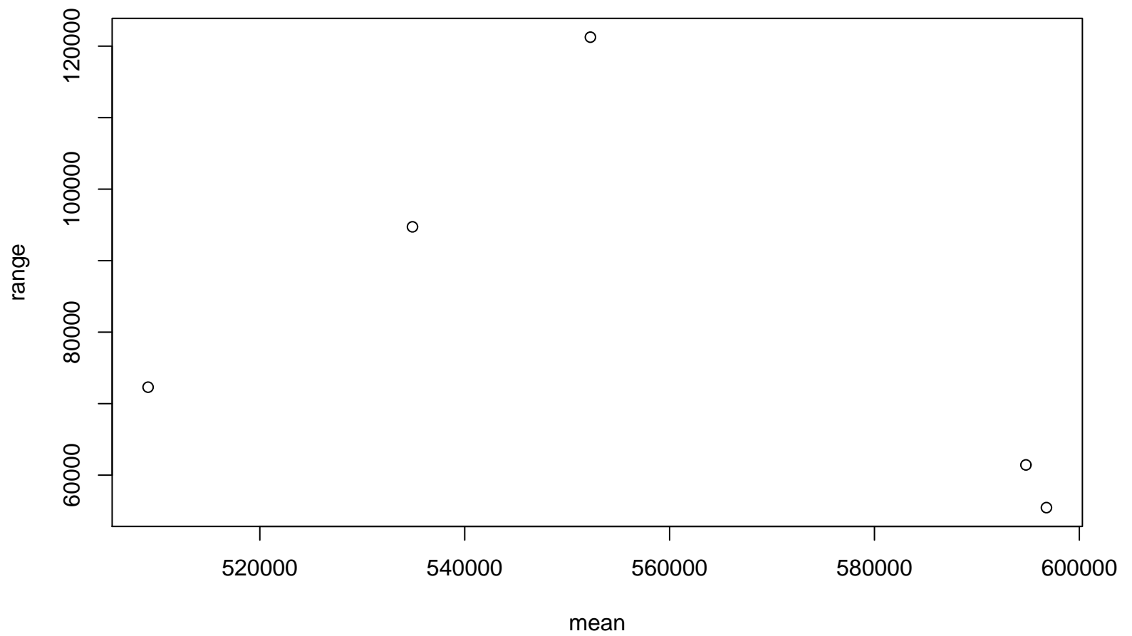
Range-Mean Plot
