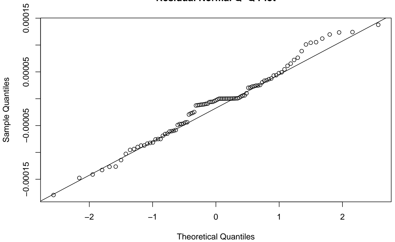
Residual Normal Q-Q Plot
