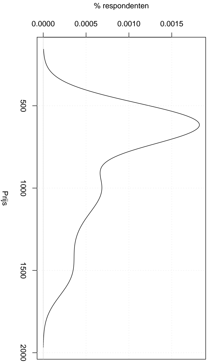
Gaussian Kernel
