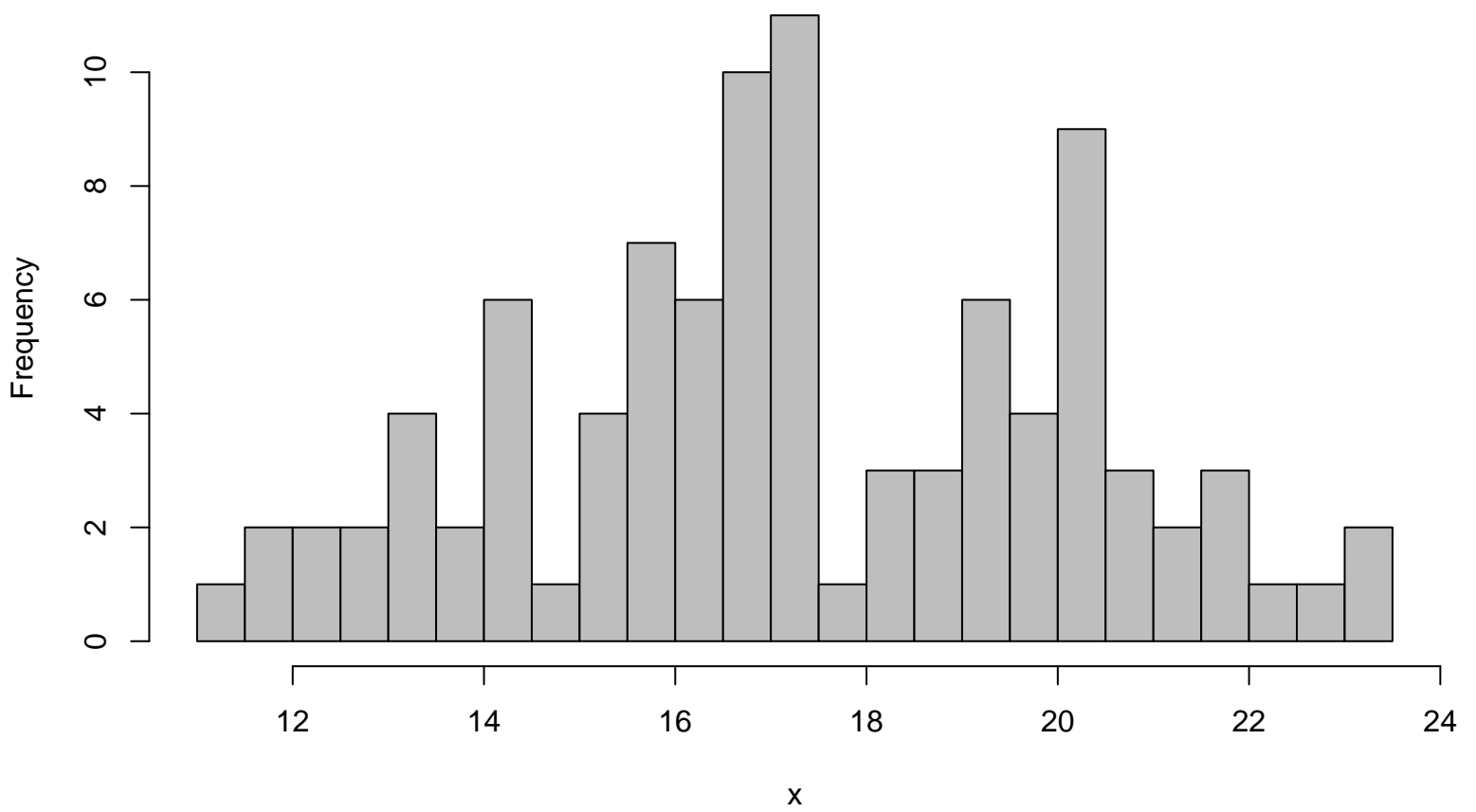
Histogram
