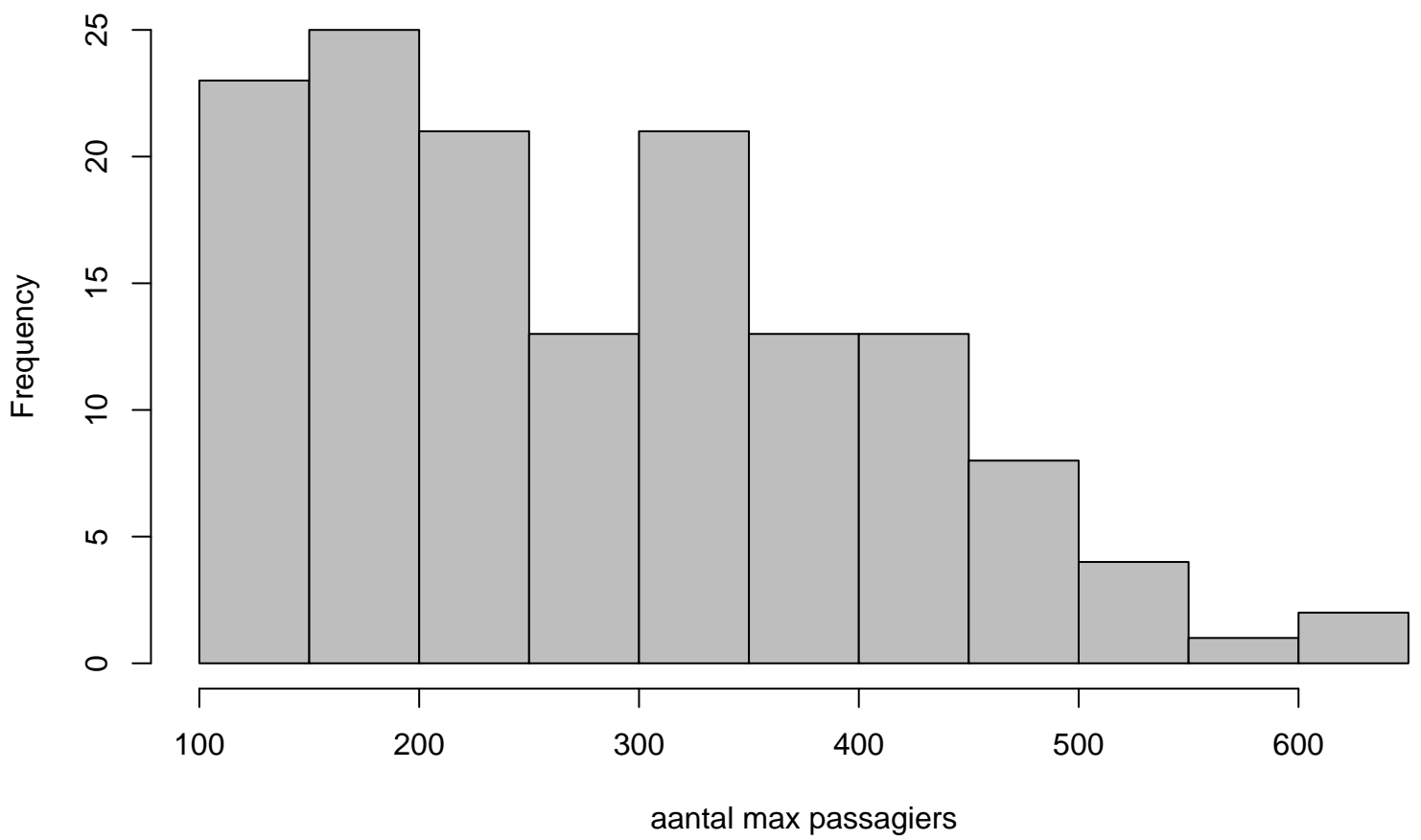
Histogram
